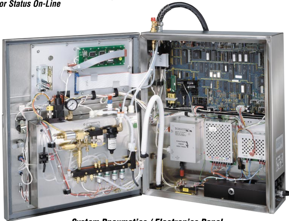
System Pneumatics / Electronics Panel
